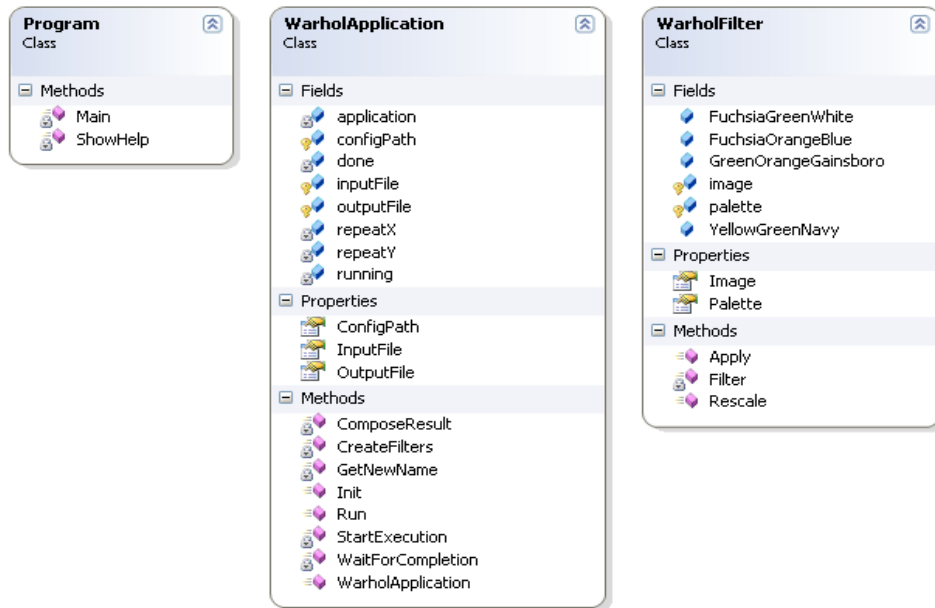
Figure 4. Class diagram.
