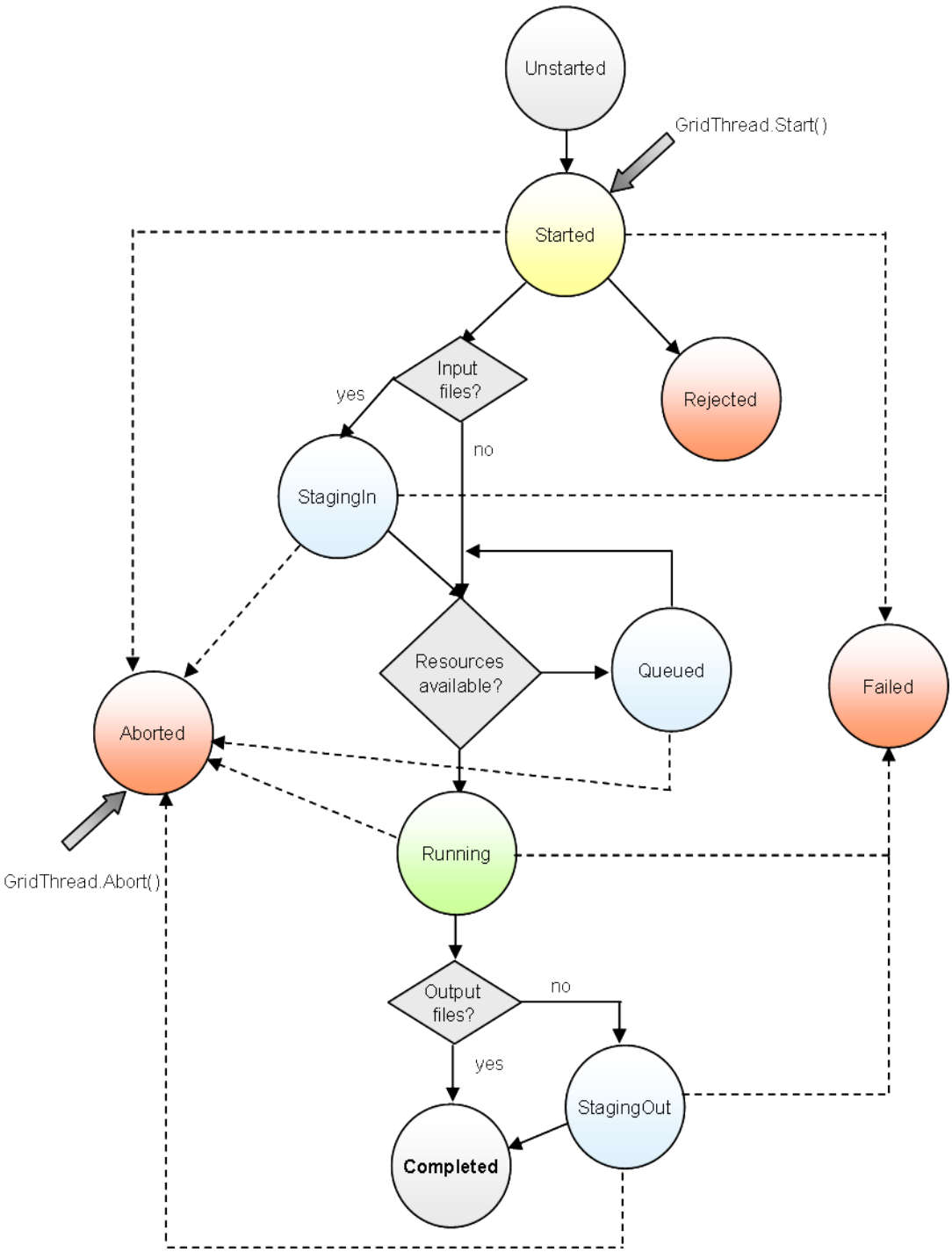
Figure 2. AnekaThread instance state transitions (client view).
