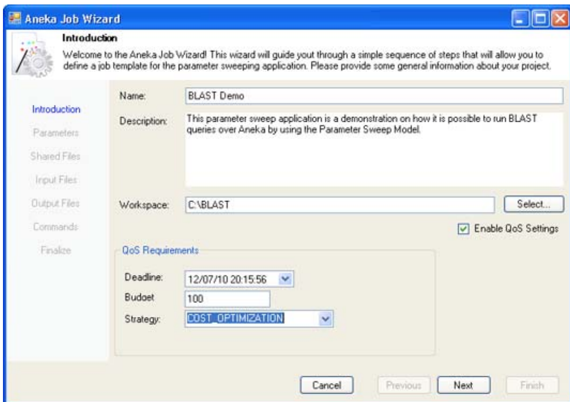
Figure 27 - Entering the Details of the BLAST Project.
